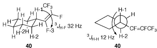
Fig. 3 Antiperiplanar coupling in Z -pentafluoropropenylcyclohexane 40 .
