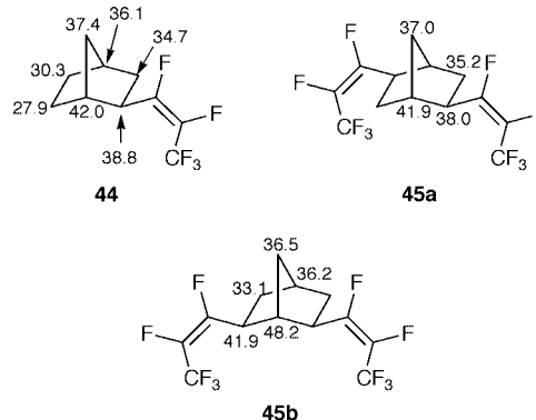
Fig. 6 ^{13}\text{C} NMR chemical shift assignments in the mono- and di-enes of norbornane.
