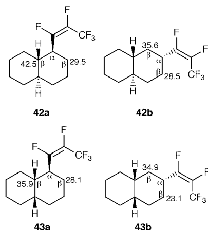
Fig. 4 ^{13}\text{C} NMR chemical shifts (ppm) of the sites \beta to fluoroalkylation in trans - and cis -decalins.
