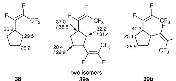
Fig. 2 13 C NMR chemical shifts (ppm) of pentafluoropropenylcyclopentane systems 38 and 39 .
