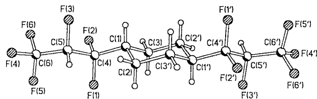
Fig. 7 X-Ray molecular structure of trans -1,4-bis(1,1,2,3,3,3-hexafluoropropyl)cyclohexane 20a . Primed atoms are symmetrically related via an inversion centre.
