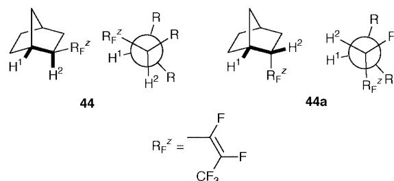
Fig. 5 Dihedral angles of exo - and endo -substituted norbornanes.
