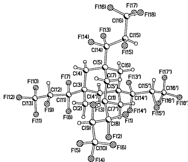
Fig. 8 X-Ray molecular structure of 1,3,5,7-tetrakis(1,1,2,3,3,3-hexafluoropropyl)adamantane 34 : one of the possible isomers ( RSSS ), the disorder is not shown. Primed atoms are symmetrically related via a mirror plane.
