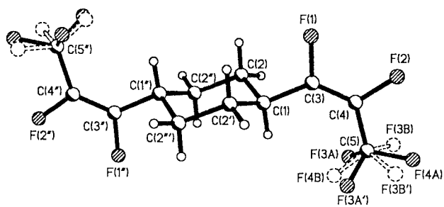
Fig. 10 X-Ray molecular structure of trans -1,4-bis[(1 Z )-pentafluoroprop-1-enyl]cyclohexane 41a . The CF 3 group is disordered over two positions with occupancies 2/3 (solid) and 1/3 (dashed). Primed atoms are related to the reference ones by m plane, double-primed by axis 2, triple-primed by the inversion centre.
