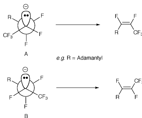
Fig. 1 Possible transition states for E1cB elimination.
