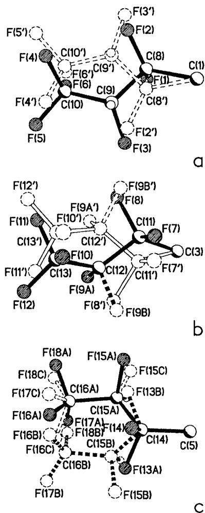
Fig. 9 Modes of disorder in RFH groups of 34 : (a) the two positions are related via a mirror plane; (b) the same, with each site shared by R and S configurations (A and B positions of F(9) have occupancies of 0.15 and 0.35, respectively); (c) symmetrically unrelated positions A ( S ) and B ( R ) have occupancies 0.7 and 0.3 respectively, with an additional rotational disorder of the former (position C, occupancy 0.2).
